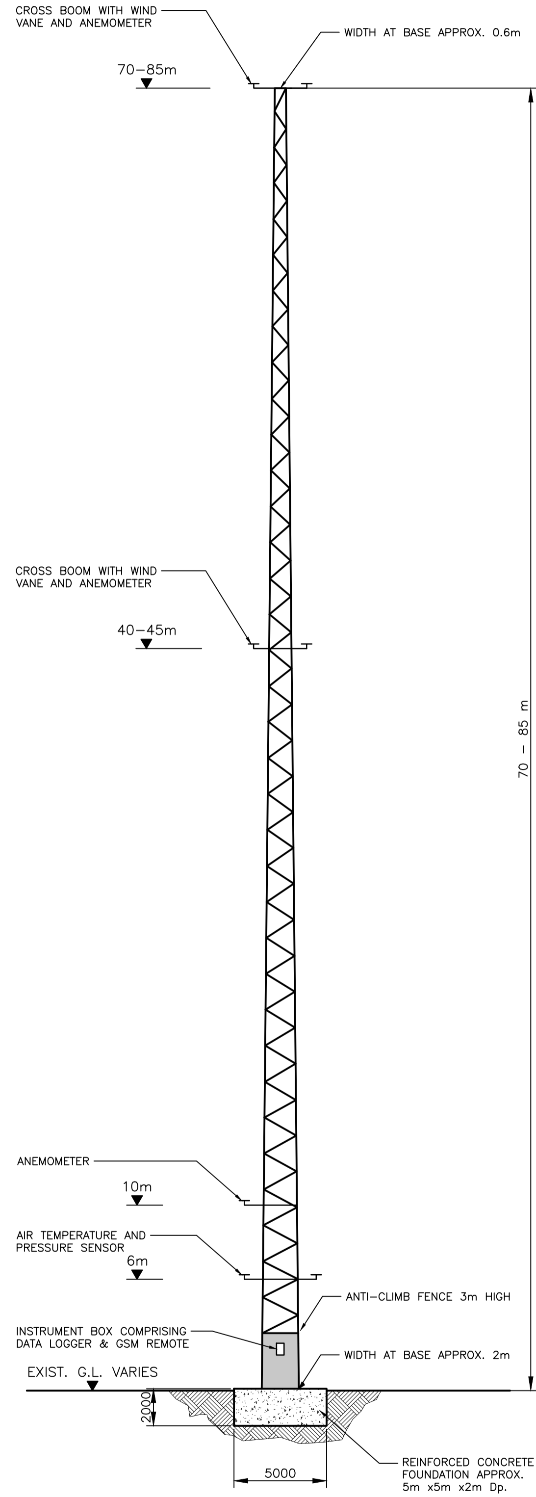
ELEVATION OF WIND MONITORING MAST N.T.S.
